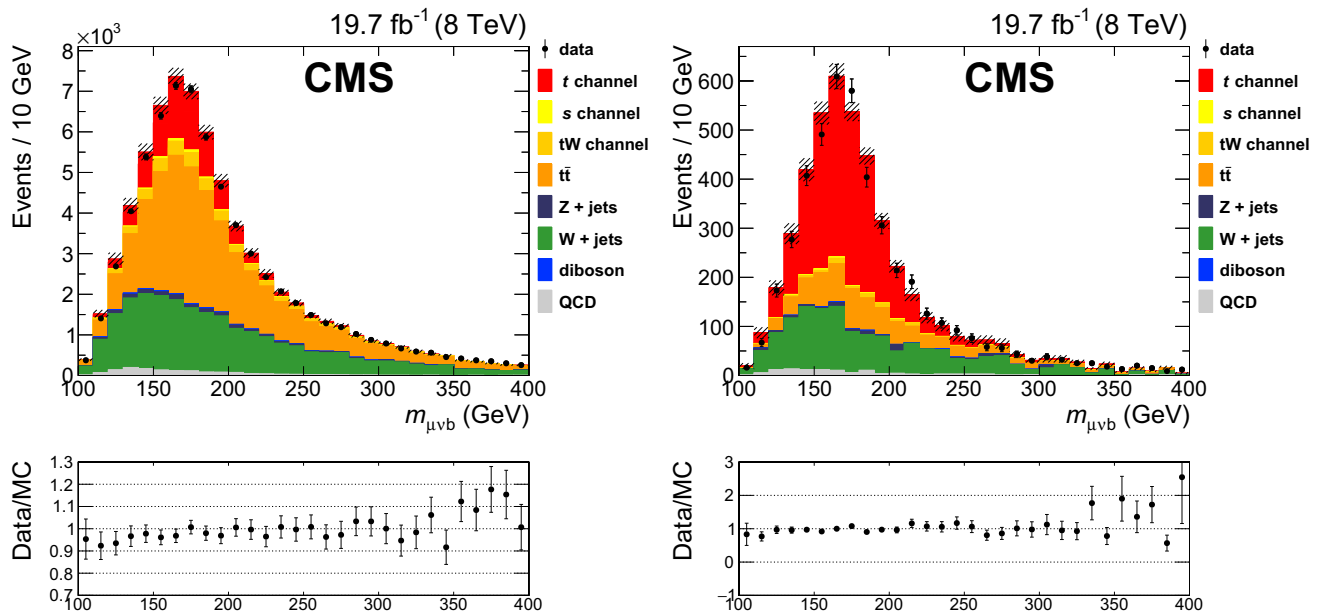
Fig. 3 Reconstructed \mu\nu b invariant mass distribution for data (points with error bars) and Monte Carlo events (stacked histograms). (Left) initial selection; (right) final selection after the charge and light-quark jet pseudorapidity requirements. The ratio of the observed number of
