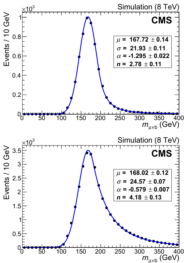
Fig. 4 Reconstructed \mu\nu b invariant mass from Monte Carlo simulated events for single top quark t channel (upper) and \bar{t}t (lower). The continuous lines show the results of fits to Crystal Ball shapes
