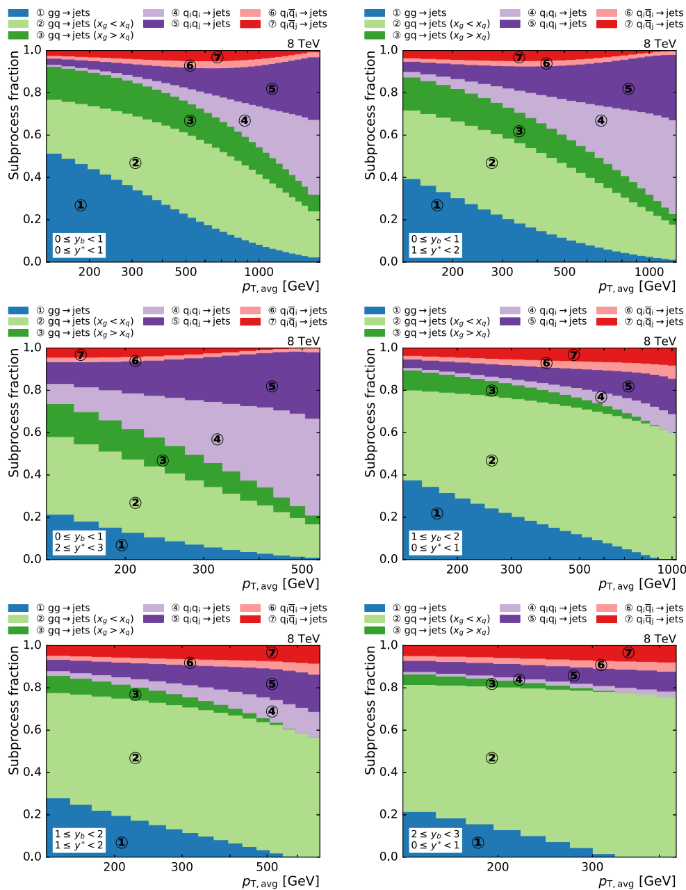
Fig. 2 Relative contributions of all subprocesses to the total cross section at NLO as a function of p_{T, \text{avg}} in the various y^* and y_b bins. The subprocess contributions are grouped into seven categories according to
