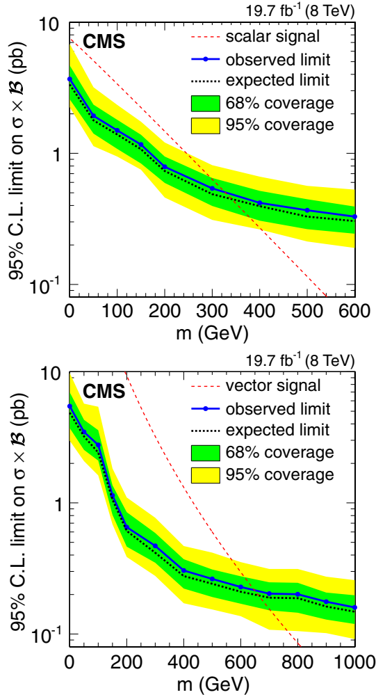
FIG. 3 (color online). The 95% C.L. expected and observed \text{CL}_s limits as functions of the mass of a scalar (top) and vector (bottom) invisible particle. The expected magnitude of a signal as a function of mass, calculated at leading order, is shown by the dashed curve. The confidence intervals for the expected limit are given at 68% and 95% coverage probability.
