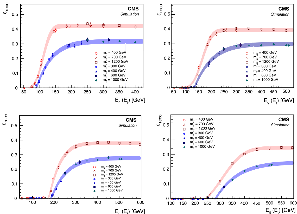
Fig. 5 The reconstruction efficiency \varepsilon_{\text{reco}} for \tilde{g} and \tilde{t} R-hadrons that stopped in the barrel region of the calorimeter as a function of the energy of the SM daughter particle for jet energy thresholds of 100, 150, 200, and 300 GeV
