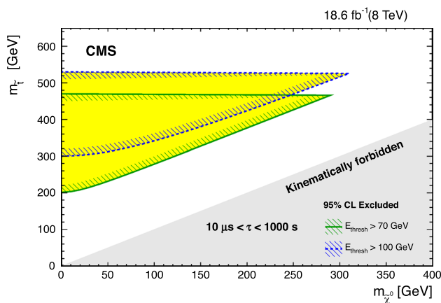
Fig. 7 Regions of the m_{\tilde{t}} - m_{\tilde{\chi}^0} plane excluded by the analysis, valid for 10^{-5} \text{ s} < \tau < 10^3 \text{ s} using two energy thresholds as indicated in the legend. The excluded regions only apply to on-shell top quarks
