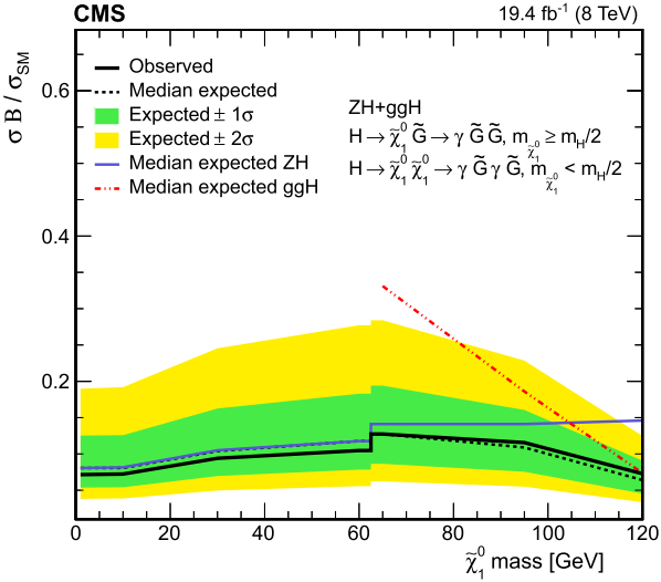
Fig. 6. Expected and observed 95% CL upper limits on \sigma_B/\sigma_{\text{SM}} for m_H = 125 GeV as a function of m_{\tilde{\chi}_1^0} assuming the SM Higgs boson cross sections, for the ZH and ggH channels and their combination, with \mathcal{B} \equiv \mathcal{B}(H \rightarrow \tilde{\chi}_1^0 \tilde{\chi}_1^0) \mathcal{B}(\tilde{\chi}_1^0 \rightarrow \tilde{\chi}_1^0 + \gamma)^2 for m_{\tilde{\chi}_1^0} < m_H/2 and \mathcal{B} \equiv \mathcal{B}(H \rightarrow \tilde{\chi}_1^0 \tilde{G}) \mathcal{B}(\tilde{\chi}_1^0 \rightarrow \tilde{G} + \gamma) for m_{\tilde{\chi}_1^0} \geq m_H/2 .
