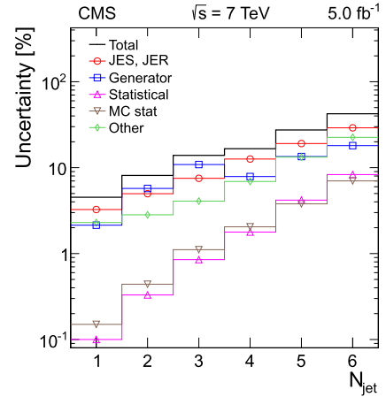
Fig. 2. The dominant systematic uncertainties in the measurement of the W + jets cross section as a function of the exclusive jet multiplicity. The systematic uncertainties displayed include the jet energy scale and resolution (JES, JER), the choice of generator used in the unfolding procedure (Generator), the statistical uncertainty in the data minus the background, propagated through the unfolding procedure (Statistical), the uncertainty due to a finite number of simulated events used to construct the response matrix (MC stat.), and all other systematic uncertainties (Other) detailed in Section 7, including pileup, integrated luminosity, background normalisation, b-tagging, muon momentum and resolution, trigger efficiency, muon identification. The uncertainties presented here correspond to the weighted average of the values shown in Table 1.
